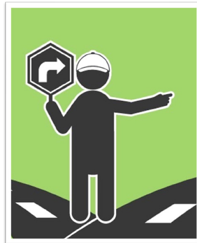
Retrain
